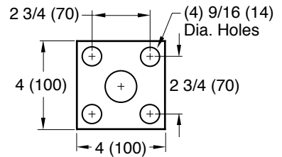
BASE DETAIL
