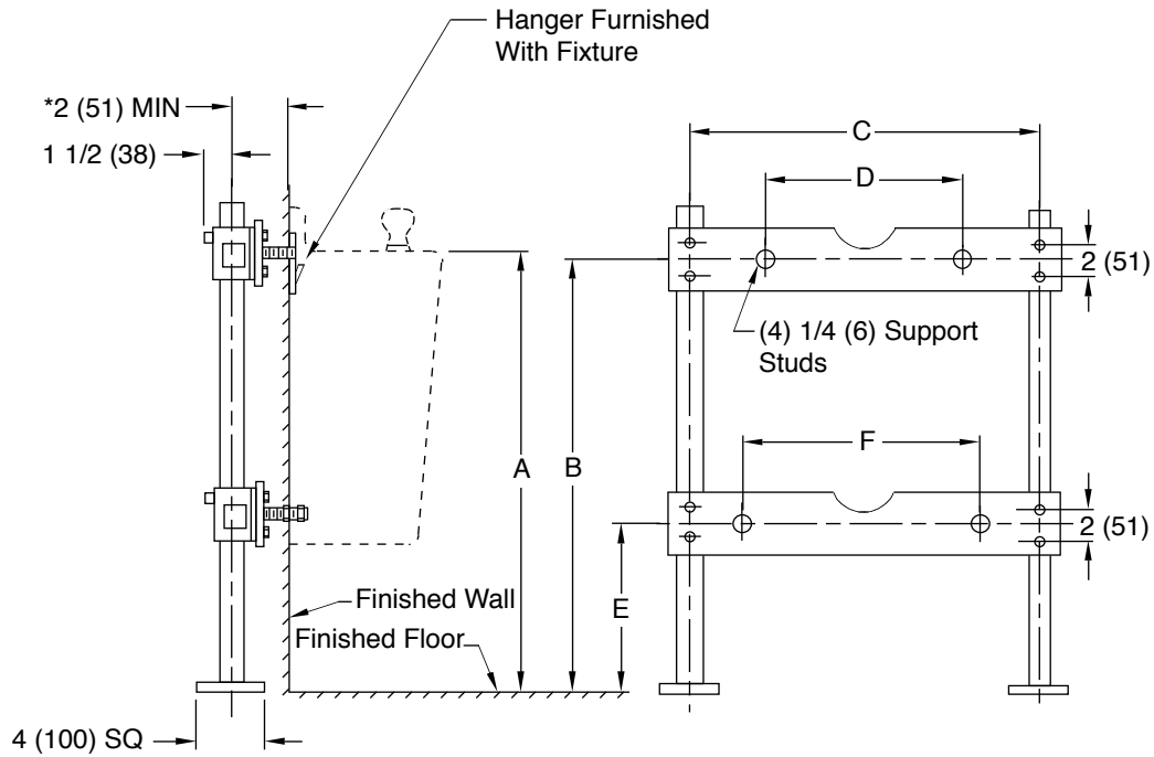
Fig. 0830 . . . FOR WALL MOUNTED ELECTRIC WATER COOLERS
