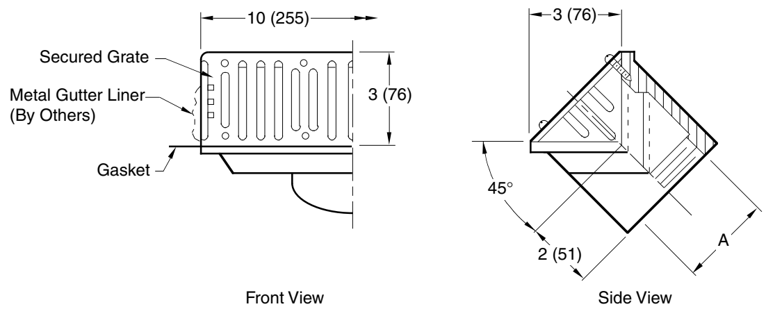
□ Fig. 1570T . . . . . 45° THREADED OUTLET A (Pipe Size) = 02(50) or 03(75)
