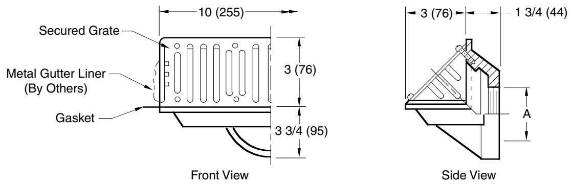
□ Fig. 1560T . . . . . 90° THREADED OUTLET A (Pipe Size) = 02(50) or 03(75)
