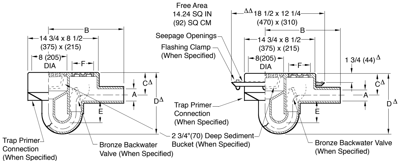
Fig. 2510S ... LESS FLANGE
