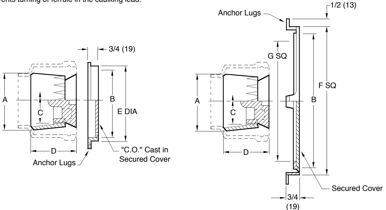
FIG. 4438C . . . . FACE-OF-WALL COVER
