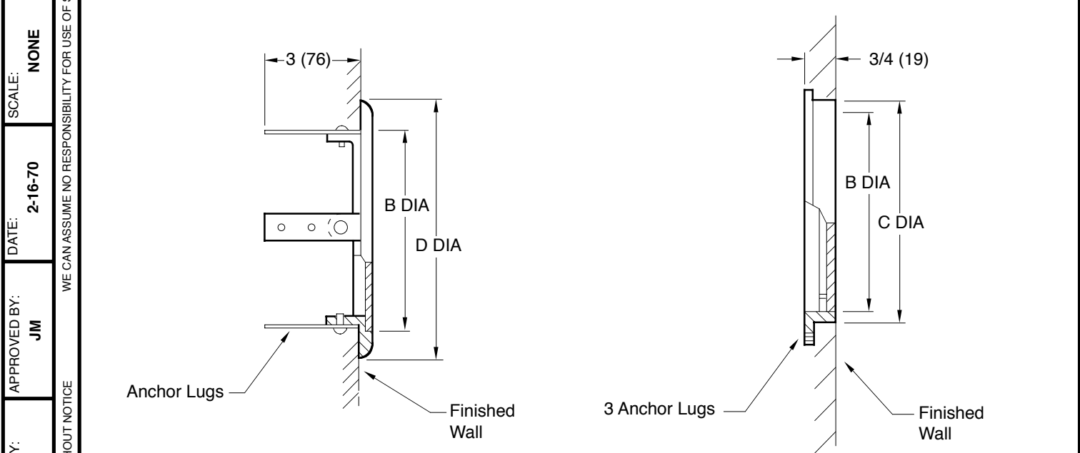
Fig. 4720 FACE-OF-WALL COVER eg: 4720 (-04)*
